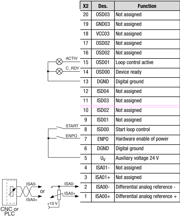
Figure 3.10 Standard terminal assignment
