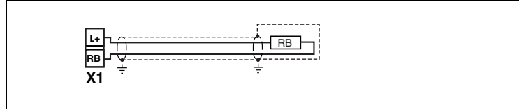
Figure 3.9 Braking resistor connection
