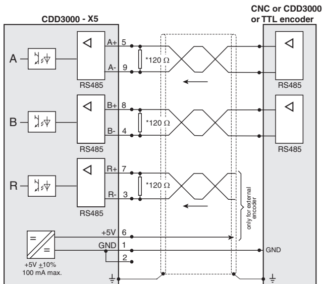
Figure 3.14 Master encoder input connection and signal description
