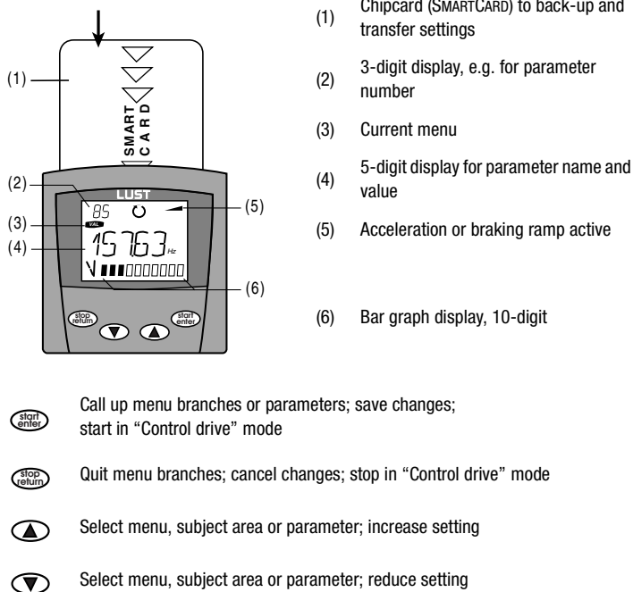
Figure 4.1 Controls and displays on the KEYPAD KP200
